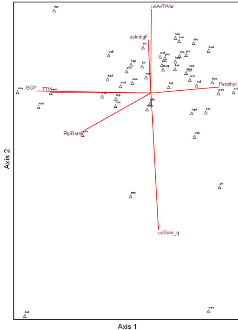
Figure 2. Non-metric multidimensional scaling axes of 46 mountain stream invertebrate communities and correlated parameters ( p < 0.01 ). Periphyt, periphyton biomass; usAveTWar, Upstream mean January air temperature; usIndigF, Percentage of upstream catchment covered in indigenous forest; TTM, total tracer movement; BCP, bottom component of Pfanckuch Index; RipBareF, Dry active channel bare of vegetation under base flow conditions; usBare_q, Percentage of upstream catchment consisting of bare ground
