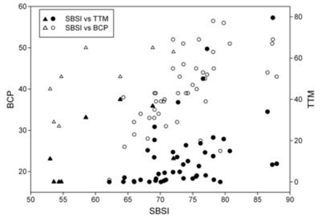
Figure 4. Site scores of the Stream Bed Stability for Invertebrates Index (SBSI) plotted against conventional measures of bed stability: In situ marked tracer stones (TTM, closed symbols) and the bottom component of the Pfankuch Stability Index (BCP, open symbols). Sites used for validation are shown as triangles
